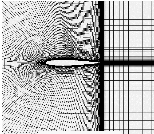
NACA0012 Airfoil Figure V
